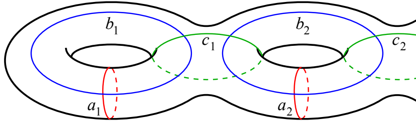
FIGURE 2. Curves used to define Dehn twists.
