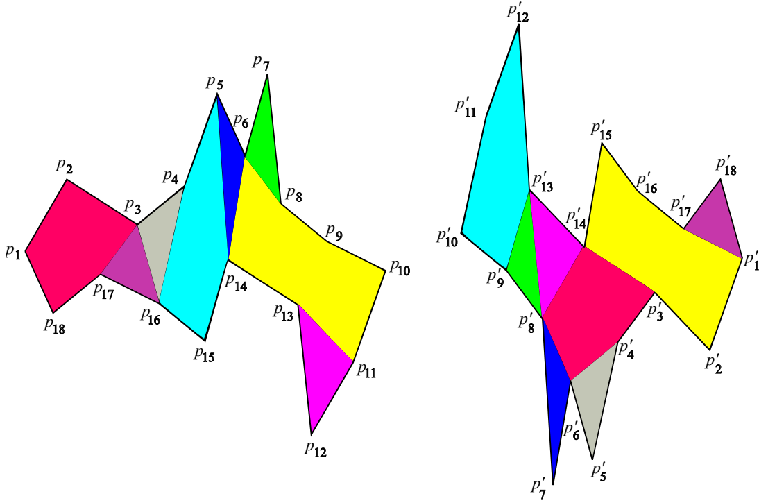
FIGURE 4. Partition of (M, q) and (M', q') = A(M, q) .
