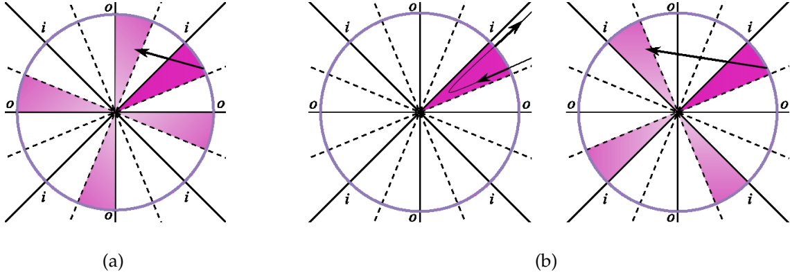
FIGURE 1. Mapping of the 4(d+1) hyperbolic sectors by \phi near a degree 2d = 6 singularity: (a) \rho(\phi_*) < 0 : the sectors are permuted and the index is 1; (b) \rho(\phi_*) > 0 : the sectors can either be fixed (left, index 1 - 2(d + 1) = -7 ) or permuted (right, index 1). The index is defined as the number of turns of a vector joining x to \phi(x) as x travels counterclockwise around a small circle. The separatrices of the unstable foliation are alternately labeled ingoing ( i ) and outgoing ( o ).
