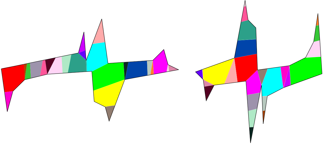
FIGURE 5. Partition of (M, q) and (M', q') = A(M, q) .
