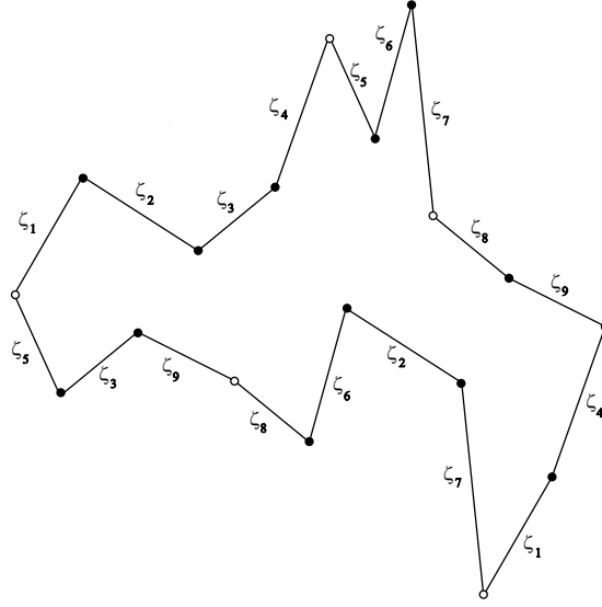
FIGURE 3. Construction of (M, q) . There are two singularities for the metric: one with conical angle 4\pi (hollow circles) and one with conical angle 12\pi (filled circles). The stratum is thus (2, 10) .
