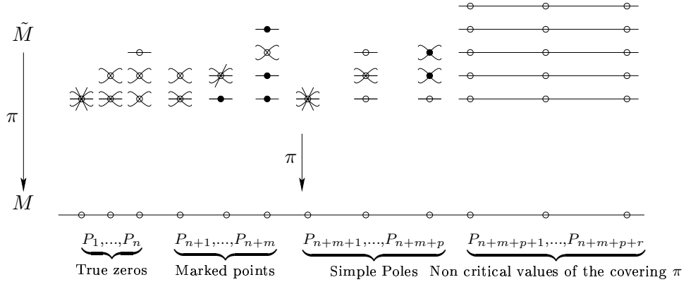
FIGURE 2. This example presents a covering of degree 5 with 21 ramification points. There are 9 critical values of \pi . Here we have n = m = p = r = 3 . The points \tilde{P} \in \pi^{-1}(P_i) which correspond to regular points of \pi^*\psi are painted in black. By convention we do not mark them.
