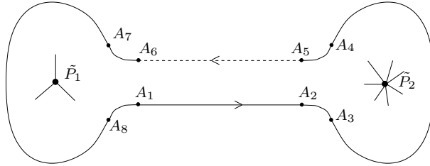
FIGURE 1. A path \tilde{\gamma} on the covering surface obtained by lifting of the path \gamma . Since \tilde{P}_1, \tilde{P}_2 \in \tilde{M} are ramification points, the segments A_1A_2 and A_6A_5 are located at the “different sheets” of the covering \tilde{M} \rightarrow M , and not nearby.
