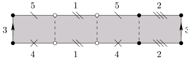
FIGURE 3. Consider the following identifications of the boundary of this polygon: identify the corresponding pairs of segments with the numbers 1, 2 and 3 by translations; identify the corresponding pairs of segments with the numbers 4 and 5 by centrally symmetries. We get a half-translation surface. In this case it has genus g = 2 and the meromorphic differential induced from the quadratic differential (dz)^2 in the plane has two zeros of order 2 on this surface. The singularities are conical point in the flat metric with a cone of angle 4\pi . Note that since the horizontal foliation is not oriented the corresponding quadratic differential is not the square of an Abelian differential, though all cone angles of the singularities in the flat metric are integer multiples of 2\pi .
