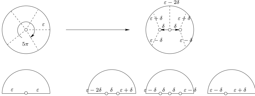
FIGURE 6. Breaking up a zero of order 3 into three zeros of orders 1. Note that the surgery is local: we do not change the flat metric outside of the neighborhood of the zero.
