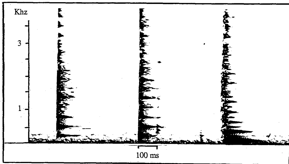
Figure 14 Transverse flute. Left to right: key click, pizzicato and tongue ram.
