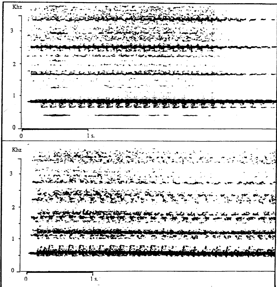
Figure 12 Shakuhachi. Two traditional ornaments. Above: karakara. Below: korokoro.
