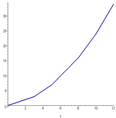
Figure 1: Newton polygons of R(X) and S(X) with respect to powers of p and X , of heights 34 and 48, resp.
