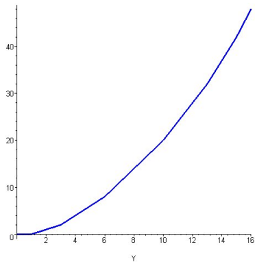
Figure 1: Newton polygons of R(X) and S(X) with respect to powers of p and X , of heights 34 and 48, resp.
