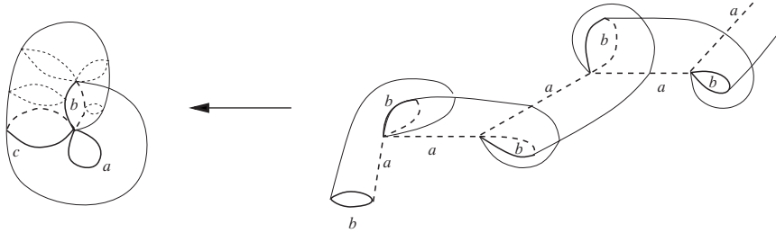
Figure 1. The universal covering \tilde{X} .
