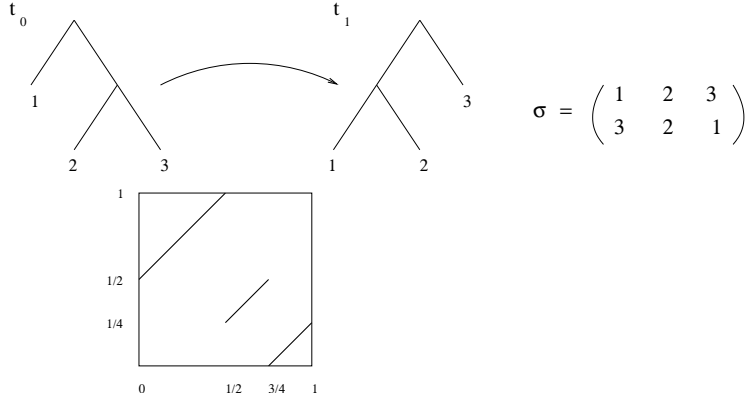
Figure 2. Symbolic representation of an element of V , with its corresponding representation as a piecewise dyadic affine bijection
