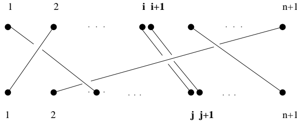
Figure 13. Diagram of strands representing the braid \partial_n^i(\sigma)
