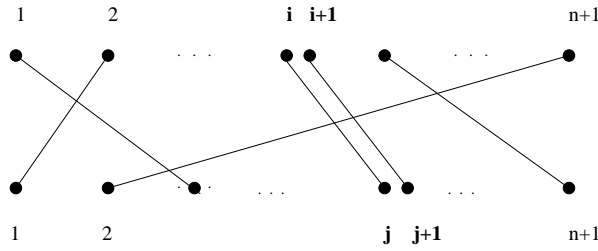
Figure 11. Diagram of strands representing the permutation \partial_n^i(\sigma)
