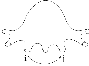
Figure 14. The mapping class \sigma \in M^*(0, n) permuting the i^{th} and j^{th} boundary circles
