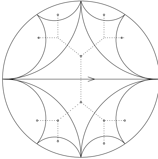
Figure 5. Farey tessellation and its dual tree
