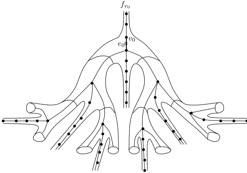
Figure 4. Decomposition of \mathcal{S}_{0,\infty}^t into pants with tubes
