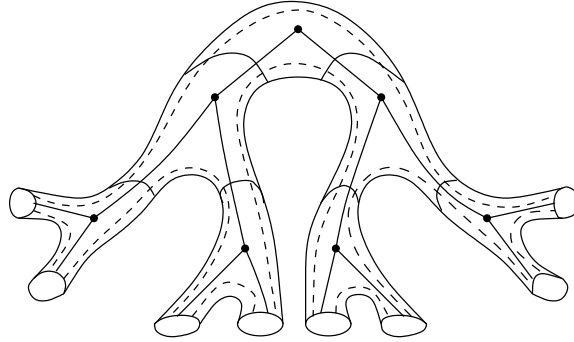
Figure 3. Surface \mathcal{S}_{0,\infty} with its canonical rigid structure
