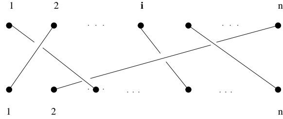
Figure 12. Diagram of strands representing a braid \sigma
