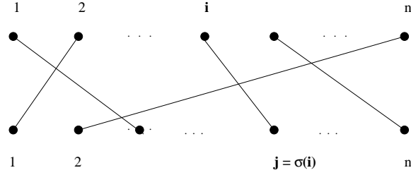
Figure 10. Diagram of strands representing a permutation \sigma
