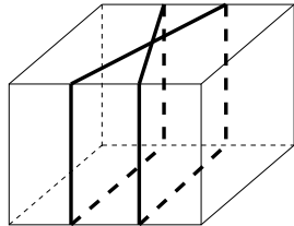
Figure 3: An immersion not extendible over the ball
