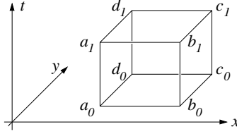
FIGURE 4. The cube \Gamma \times [0, 1] in \mathbf{C} \times \mathbf{R}
