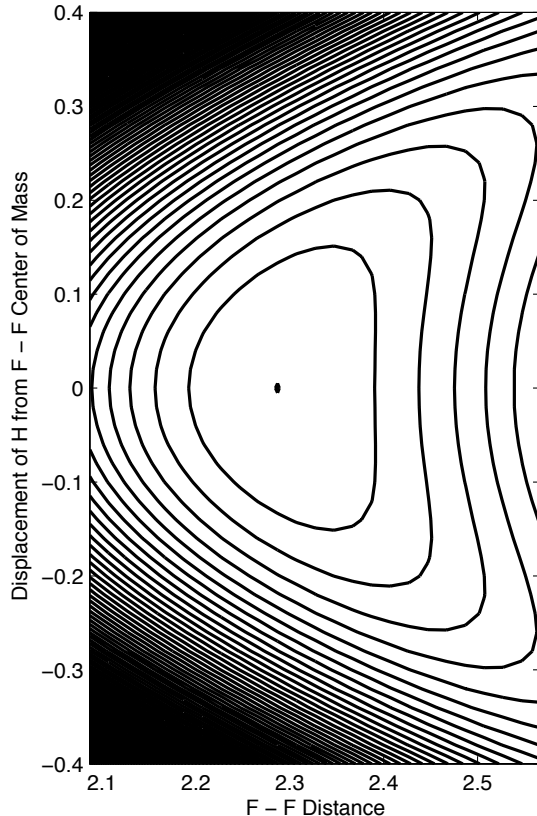
Figure 1: Contour plot of the ground state electronic potential energy surface in the Jacobi coordinates (W, Z) . It is obviously not well approximated by a quadratic. Our technique exploits the flatness of the surface in the Z direction near the minimum.
