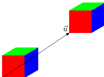
FIGURE 10. Translation
