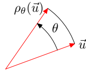
FIGURE 9. Rotation vectorielle
