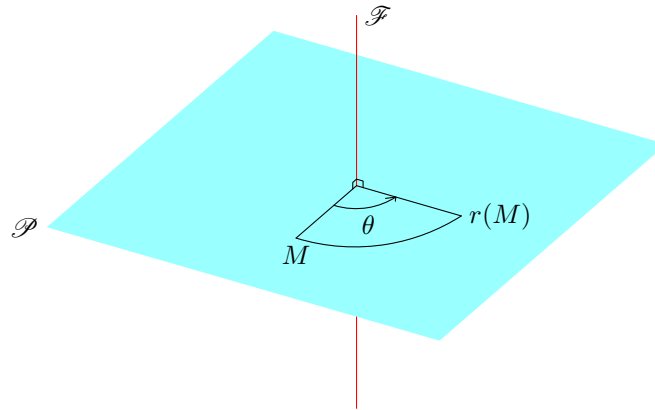
FIGURE 12. Rotation affine
