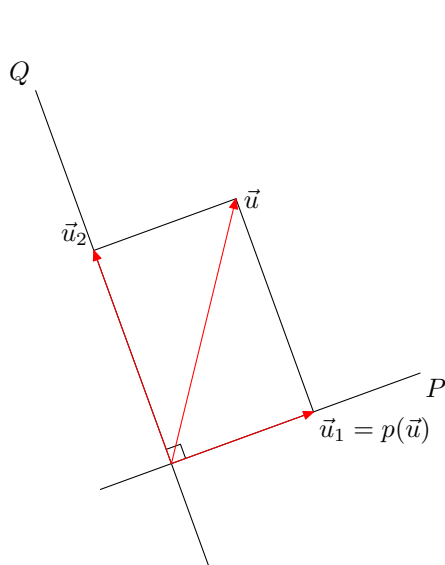
FIGURE 7. Projection orthogonale
