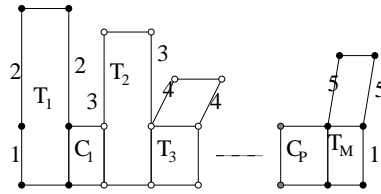
FIGURE 5. The tori and cylinders are cyclically glued to a “necklace” where two ‘neighboring’ tori might be glued directly or by a cylinder in between them.
