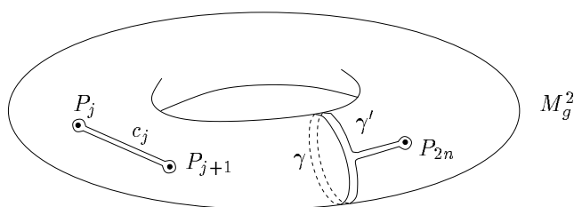
Figure 4: The points P_j, P_{j+1} , and P_{2n} of the underlying surface M correspond to singularities of \psi of odd degree. The paths \gamma and \gamma' are homologous in H_1(M; \mathbb{Z}_2) , but holonomy along \gamma and along \gamma' is different. Holonomy along the path c_j is obviously trivial.
