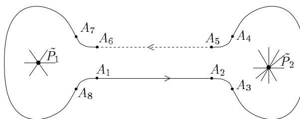
Figure 5: A path \tilde{c}_j on the covering surface obtained by lifting the path \tilde{c}_j . Since \tilde{P}_j, \tilde{P}_{j+1} \in \tilde{M} are ramification points, the segments A_1A_2 and A_6A_5 are located on “different sheets” of the covering \tilde{M} \rightarrow M , and are not near to one another.
