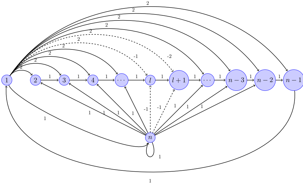
FIGURE 8. The graph associated to V_{n,k} . In dashed line we have represented arrow that need to be removed from the graph in blue. Multiplicity are also indicated. To be more more precise, there is one arrow from vertex labelled 1 to the vertex labelled l and no arrow from vertex labelled 1 to the vertex labelled l+1 . In the graph l = \lfloor \frac{i(n-1)}{k} \rfloor + 1 for any i = 1, \dots, k-1 . Obviously the graph associated to A_n is drawn in blue colour
