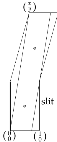
FIGURE 2. A cylinder fixed by the elliptic involution on a slit torus
