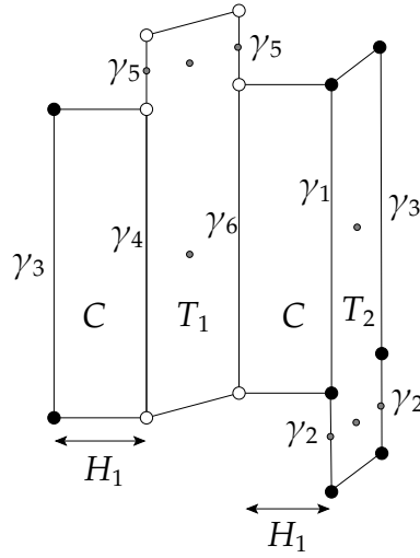
FIGURE 13. The decomposition of (X_n, \omega_n) in the direction \Theta : this is a completely periodic 2T_{\text{fix}}2C -direction.
