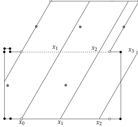
FIGURE 12. A periodic direction on (X_3, \omega_3) in the direction \Theta .
