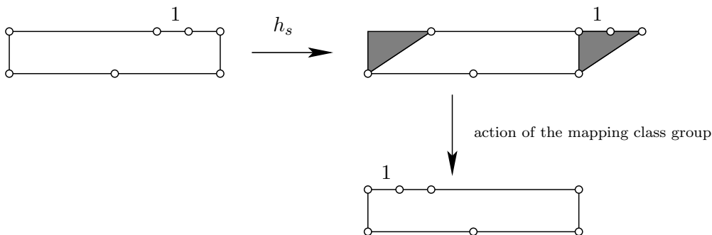
FIGURE 4. Action of the horocyclic flow h_s on a flat surface.
