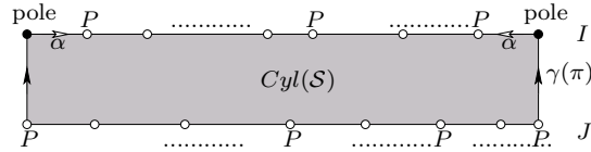
FIGURE 11. A flat surface with a unique zero and a unique pole.
