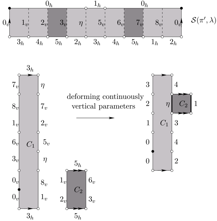
FIGURE 12. A flat surface \mathcal{S}' = \mathcal{S}(\pi'\lambda_0) suspended over the permutation \pi' and the admissible vector \lambda_0 (see Equation (7.1)). The vertical foliation decomposes \mathcal{S}' in two cylinders C_1 and C_2 . The cylinder C_2 is a simple cylinder: the conical angle of its boundary \eta is \pi . Moreover the length of \eta can be chosen arbitrary small with respect to other vertical parameters: C_2 has multiplicity one.
