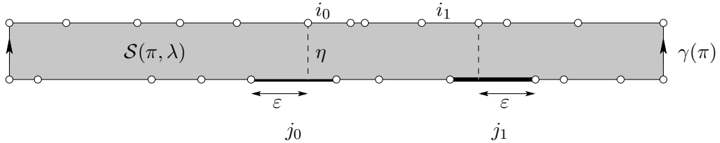
FIGURE 6. A separatrix of length 2 (here the canonical separatrix \gamma(\pi) has length 1). The two corresponding horizontal intervals of length \lambda_{j_0+r} and \lambda_{j_1+r} , labelled by j_0 and j_1 , are glued by a central symmetry.
