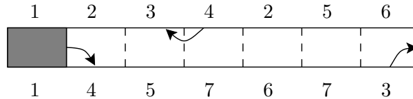
FIGURE 8. A vertical decomposition on a flat surface representing the component \mathcal{Q}^{irr,I}(12) .
