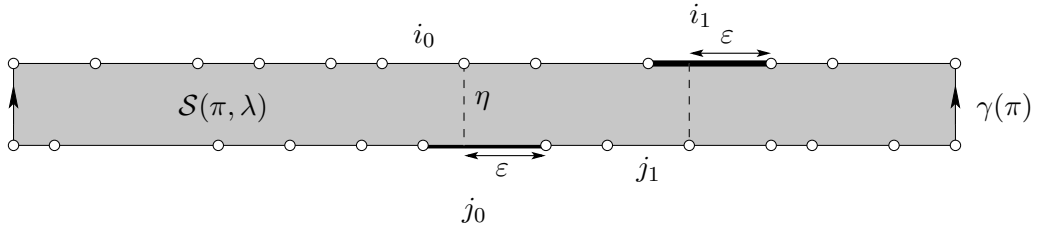
FIGURE 5. A separatrix of length 2 (here the canonical separatrix \gamma(\pi) has length 1). The two corresponding horizontal intervals of length \lambda_{j_0+r} and \lambda_{i_1} , labelled by j_0 and i_1 , are glued by a translation.
