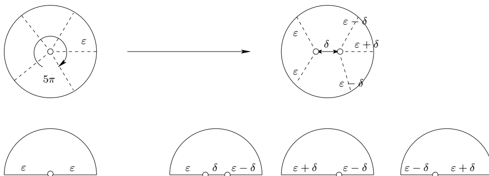
FIGURE 1. Breaking up a zero of order 3 in two zeroes of orders 1 and 2 correspondingly. Note that the surgery is local: we do not change the flat metric outside of the neighborhood of the zero.
